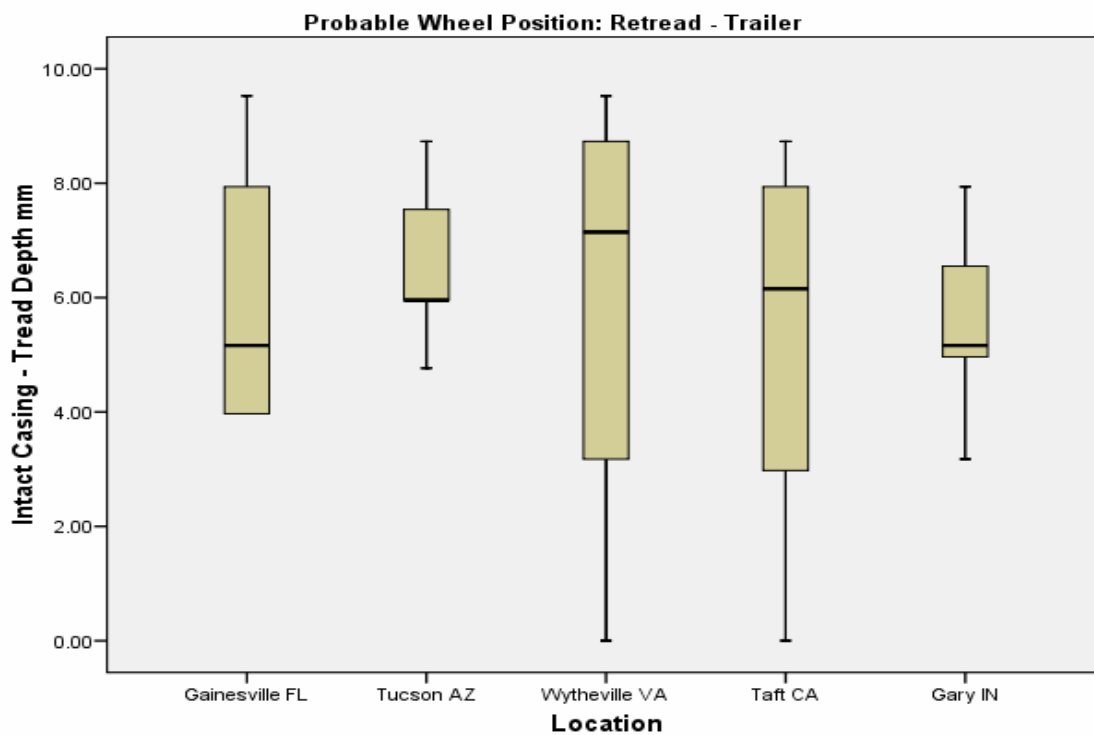
Retread Trailer Wheel Position by Tread Depth and Collection Location (n=40)
