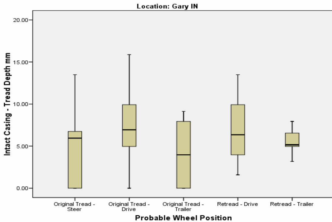
Gary IN Probable Wheel Position and Intact Casing Tread Depth (n=39)
