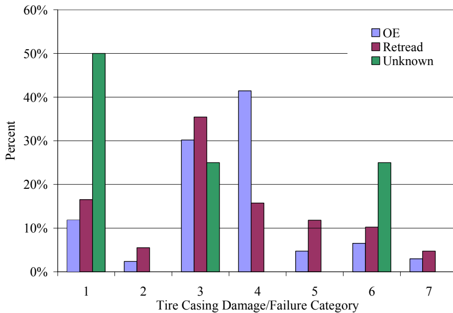
Figure 9.24 - Tire Casings Damage/Failure Category Determination
