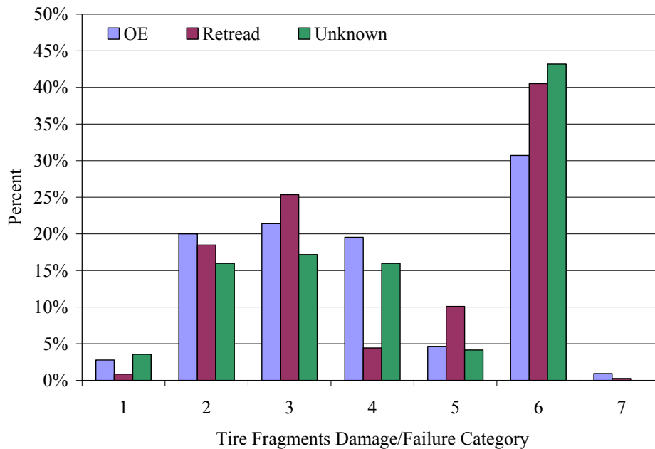
Figure 9.25 - Tire Fragments/Debris Damage/Failure Category Determination
