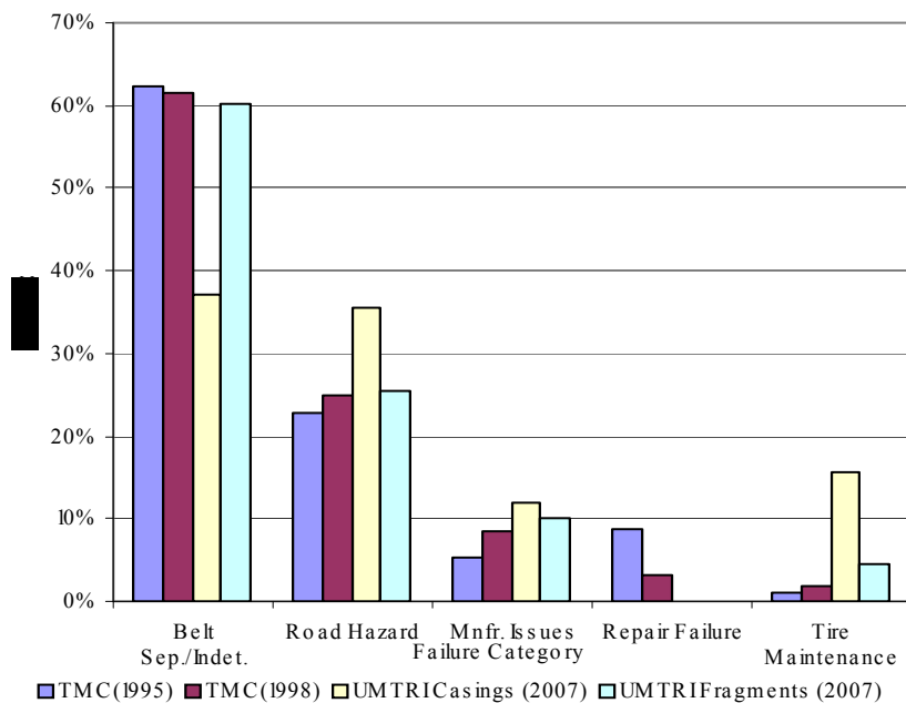
Figure 9.39 - Failure Category Study Comparison Retread Tires
