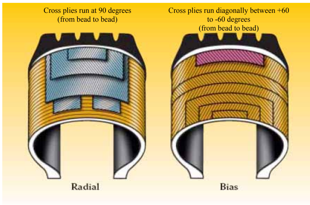
Figure 2.3 – Radial versus Bias-Ply Tire Structures
