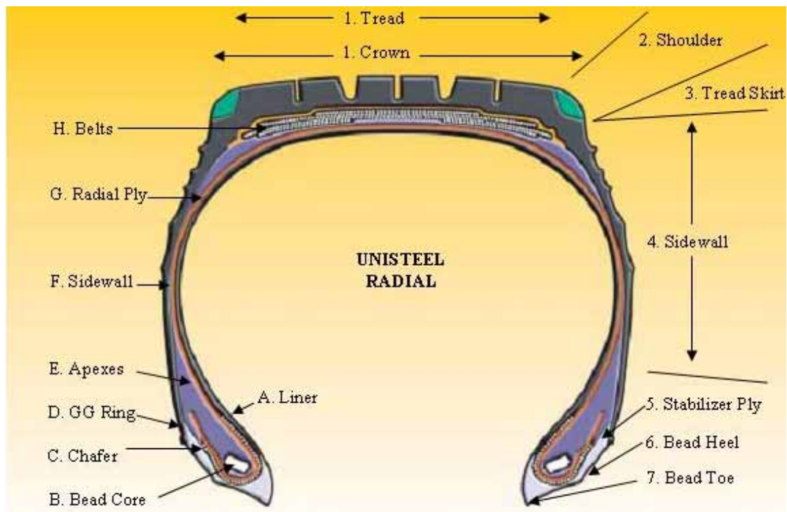
Figure 2.2 – Tire Structure
