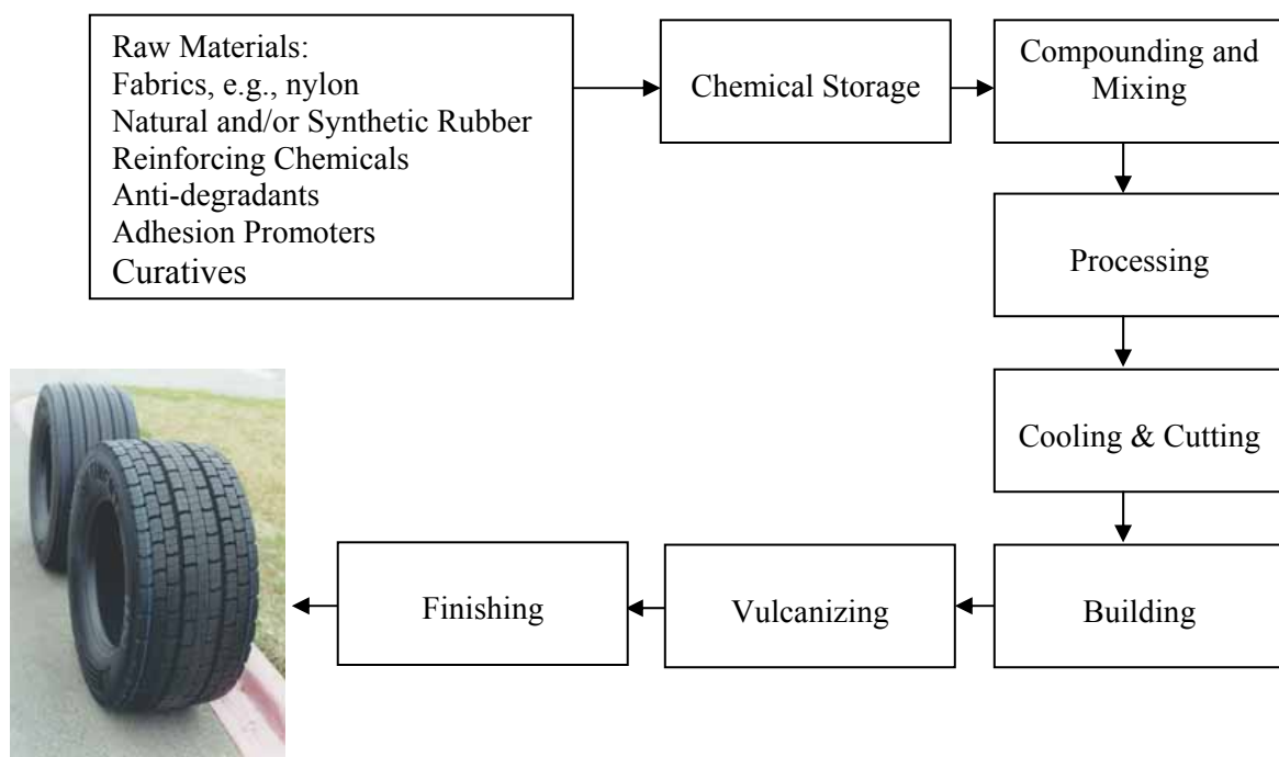
Figure 2.1 - The Tire Manufacturing Process
