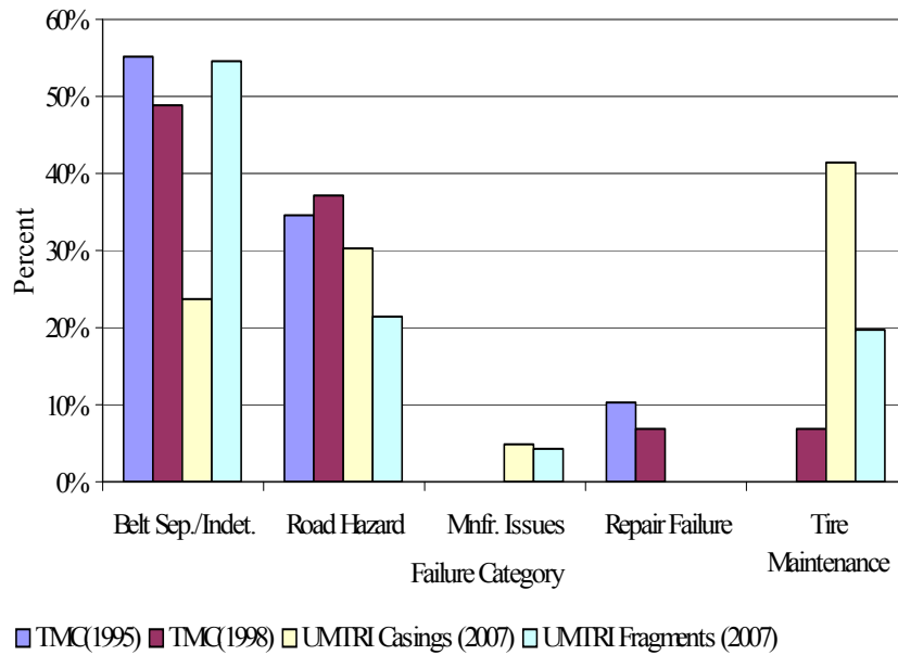
Figure 9.38 - Failure Category Study Comparison OE/New Tires
