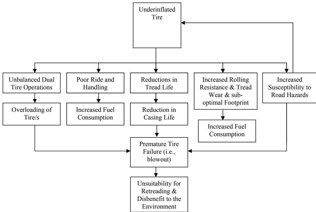
Figure 5.3 – Potential Negative Impacts Resulting From Tire Underinflation
