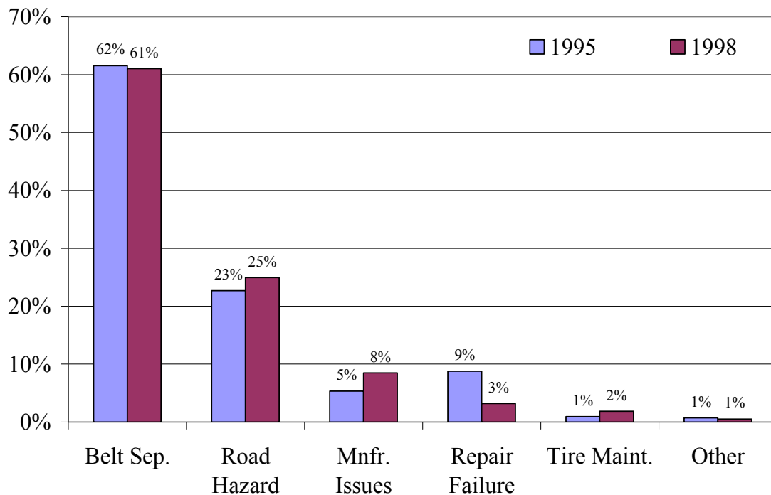
Figure 3.4 – Probable Failure Reasons Retread Tires TMC Study, 1995 & 1998
