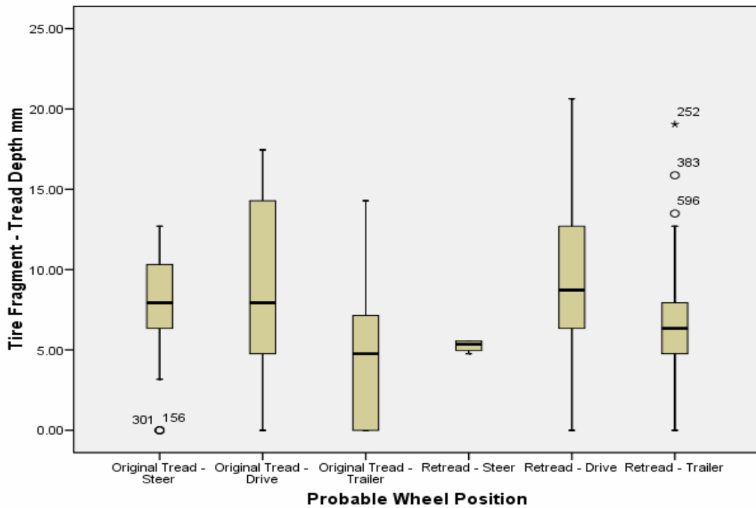
Figure 9.35 – Tread Depth by Wheel Position and Tire Fragment Status (n=890)
