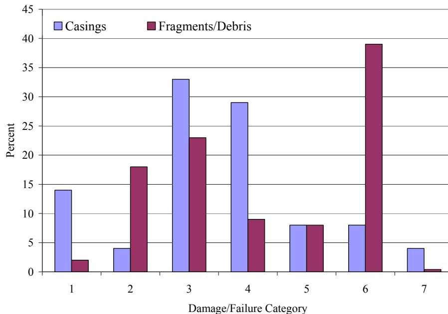
Figure 9.22 - Tire Casings & Fragments Damage/Failure Category Determination
