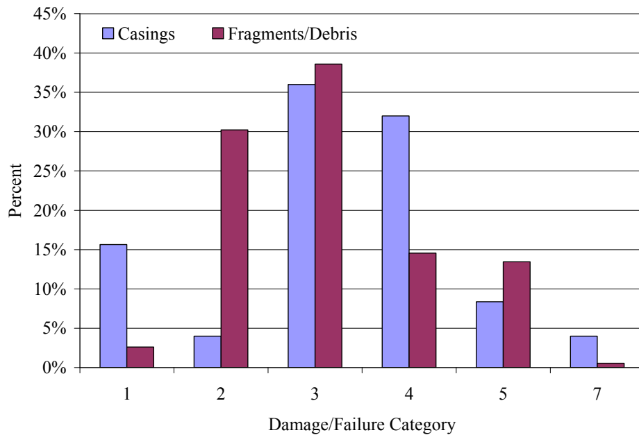
Figure 9.23 - Tire Casings & Fragments Damage/Failure Category Determination (Excluding Indeterminate Category)
