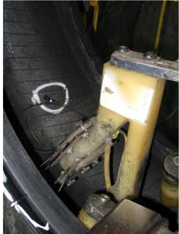
Figure 2.7 – Shearographer at Work
