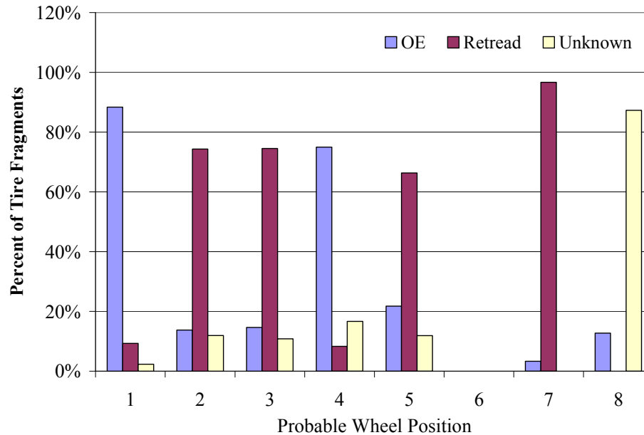
Figure 9.30: Probable Wheel Position and Tire Status (Tire Fragments)
