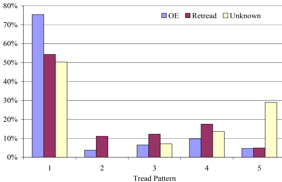
Figure 9.32 – Tire Fragment Status by Tread Pattern
