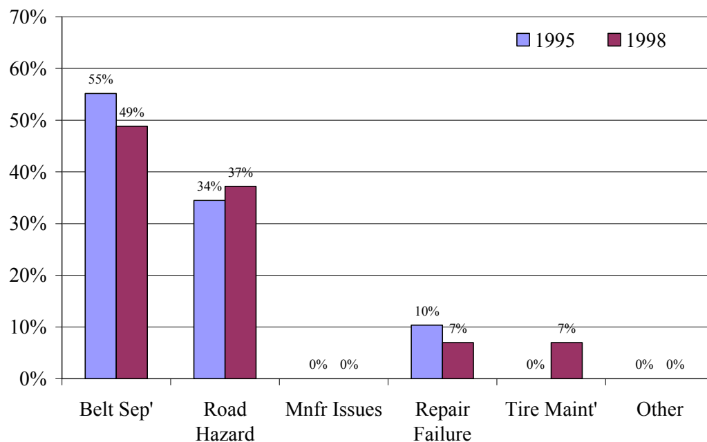
Figure 3.3 – Probable Failure Reasons New Tires TMC Study, 1995 & 1998
