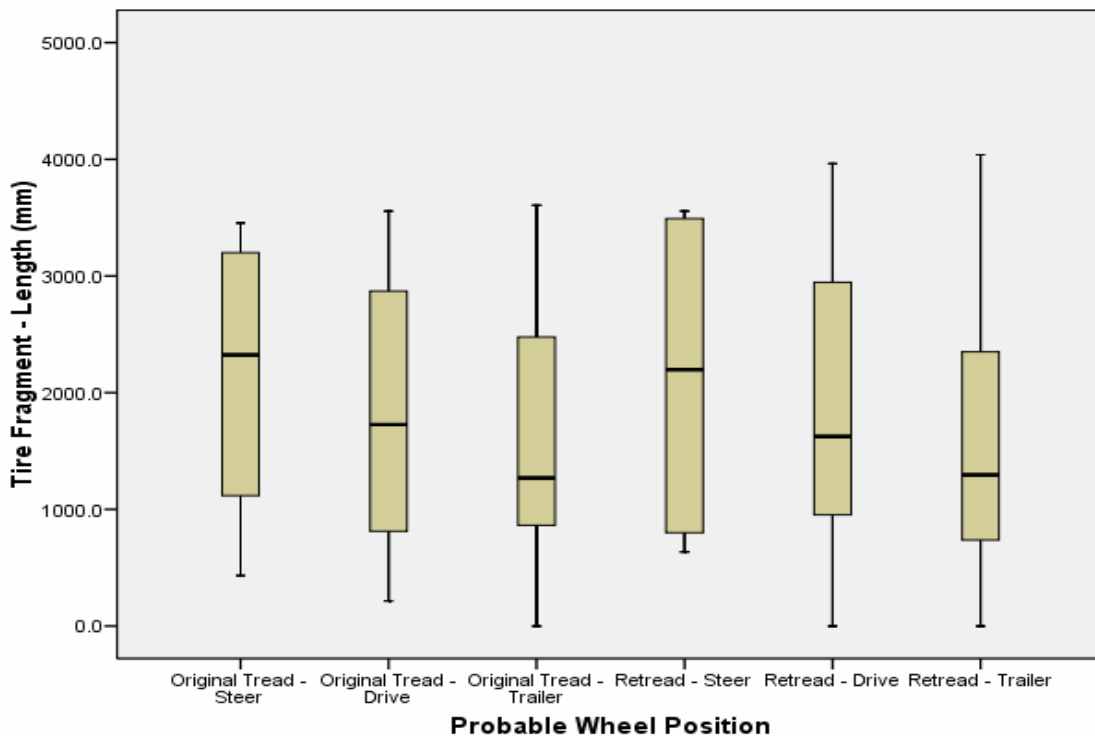
Figure 9.36 – Tire Fragment Length by Probable Wheel Position (n=890)
